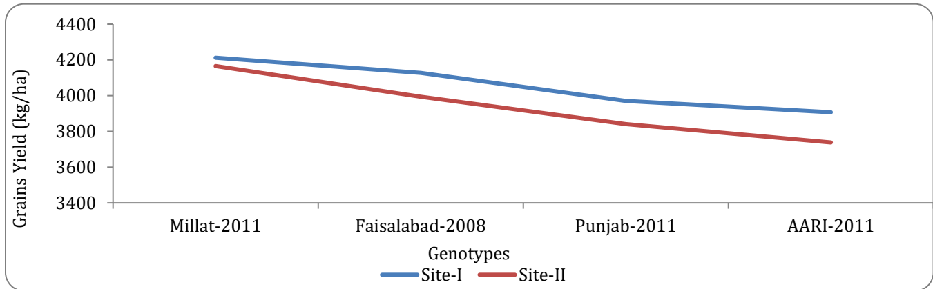
Figure 2. Correlation of grains yield (kg ha -1 ) with different genotypes sown in varying environments.
