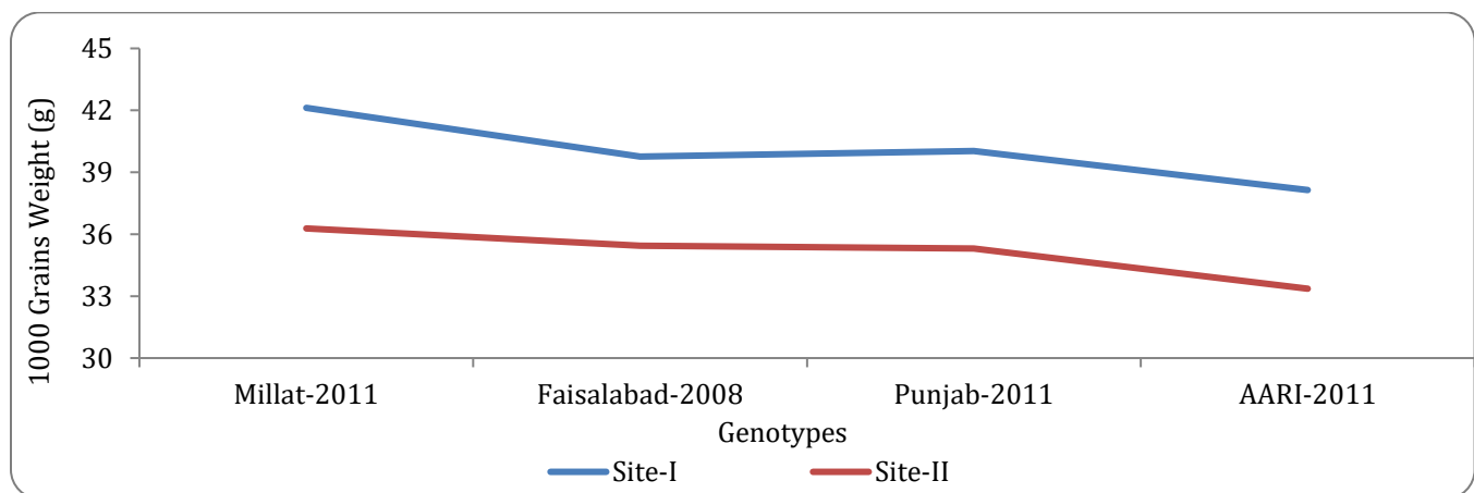
Figure 1. Correlation of 1000 grains weight (g) with different genotypes sown in varying environments.
