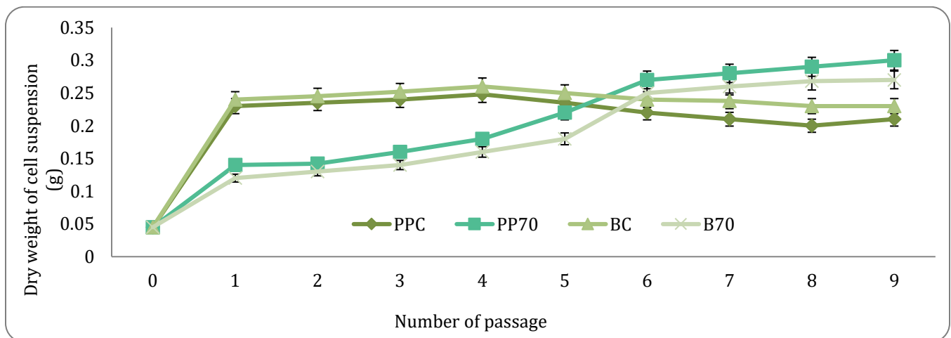
Figure 6. Long term effects of high NaCl (70 mM) on cell suspension growth of the rice cultivar Pute Perak (PP) and Basmati-370 (B-370). The duration of each passage was 12 days. PPC: Control treatment of Puteh Perak, PP70: Salinity treatment of Puteh Perak, BC: Control treatment of Basmati-370 and B70: Salinity treatment of Basmati-370.
