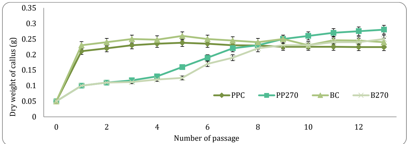
Figure 5. The long term effects of high NaCl (270 mM) on callus growth of the Pute Perak (PP) and Basmati-370 (B-370) rice cultivars. The duration of each passage was 18 days. PPC: Control treatment of Puteh Perak, PP270: Salinity treatment of Puteh Perak, BC: Control treatment of Basmati-370 and B270: Salinity treatment of Basmati-370.
